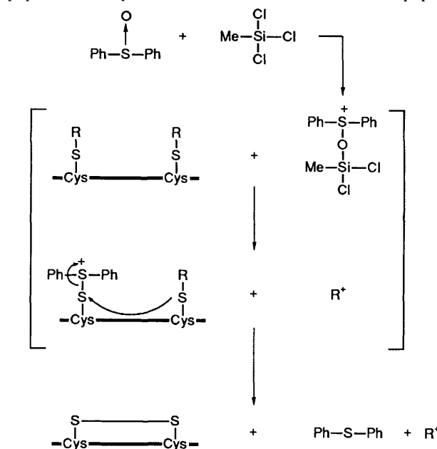
Fig. 1 Proposed pathway for the synthesis of cystine-peptide using silylchloride–sulphoxide system
